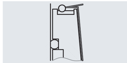
O-ring/flat gasket
